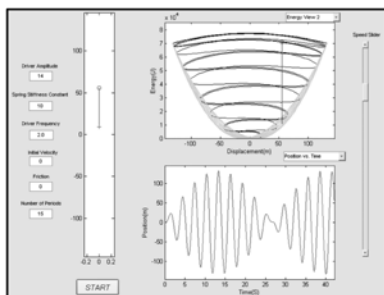
Student-written GUI Tool
