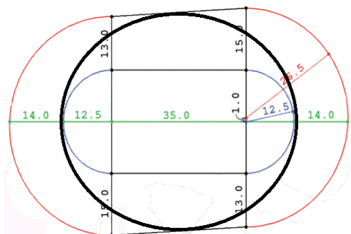
Figure 2: This image shows the dimensions of the Regulation track of the Women's Flat Track Roller Derby Association < wtdfa.com >, all dimensions are in feet. The thick black line shows a circular path skated for speed measurements. (Image after < rules.wtdfa.com/ > with author modifications).
