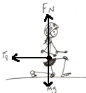
Figure 10: A traditional simplified Free Body Diagram (FBD) for a one knee fall, re-locating all forces at the CM of the skater.
